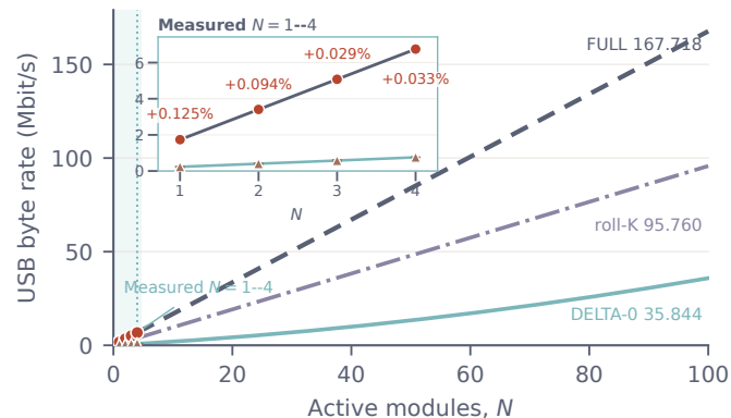
(b) USB application rate at 200 Hz
